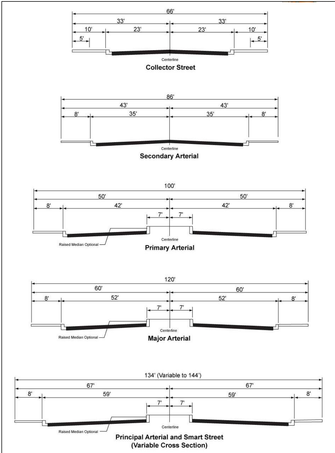
Figure CM-1 Roadway Cross Sections
